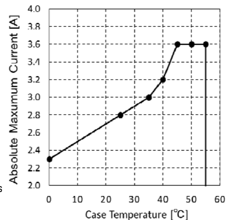
Fig.1 Absolute maximum ratings of operating current
